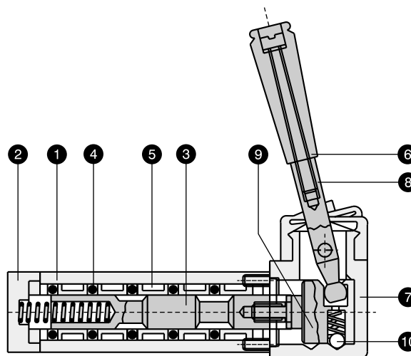
5/2 Hand Lever Actuated Modular Spool Valve
