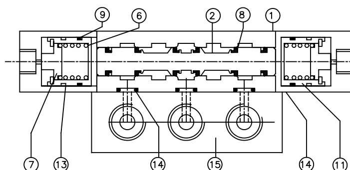
5/3 DOUBLE PILOT VALVE
