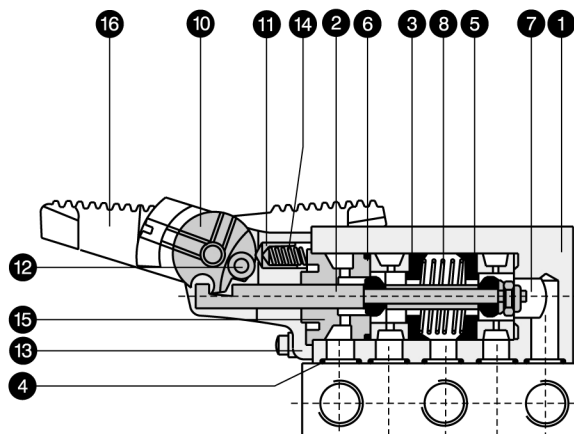
Foot Lever Operated Poppet Valve
