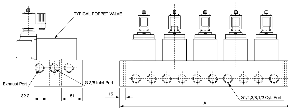
Gang Manifold - 3/8" Basic Poppet Valves
