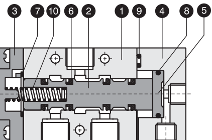
3/2 Single Pilot High Flow Valve
